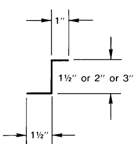
"Z" Closure
