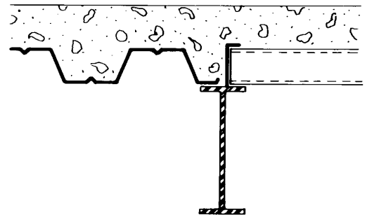
CELL CLOSURE
