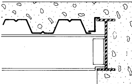
"z" CLOSURE
