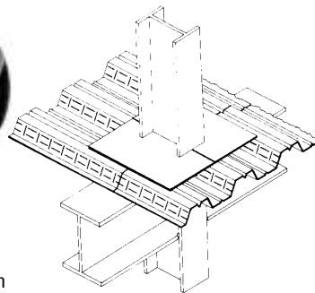
COLUMN CLOSURE
