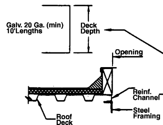
REINFORCING CHANNEL
