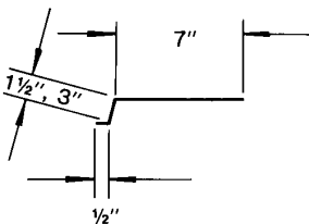
FILLER SHEET (20 GA.) 10'-0" LENGTHS GALVANIZED ONLY
