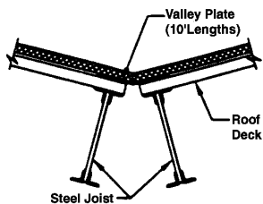
VALLEY DETAIL
