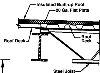
DETAIL WHERE DECK CHANGES DIRECTION
