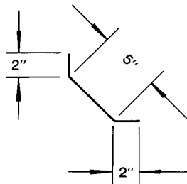
CANT STRIP (20 GA.) 10'-0" LENGTHS GALVANIZED ONLY
