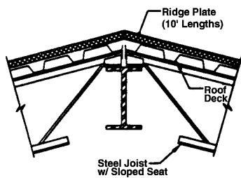
RIDGE DETAIL
