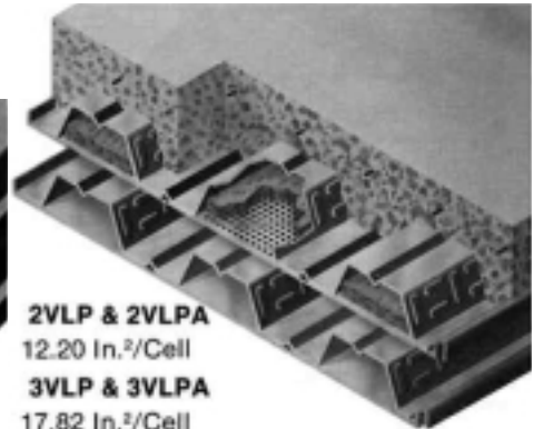
1.5VLP & 1.5VLPA 5.71 In. 3 /Cell
