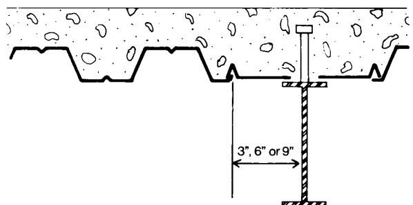
GIRDER FILLER
