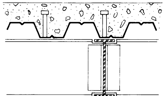
STUD LOCATIONS
