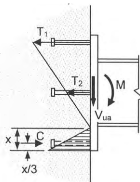
Example of simplified elastic load distribution in a beam-wall connection
