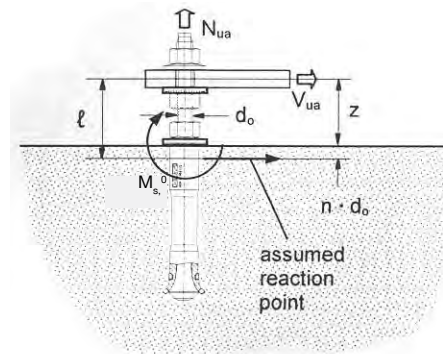
Determination of bolt bending – strength design
