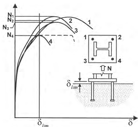
Example of deformational incompatibility
