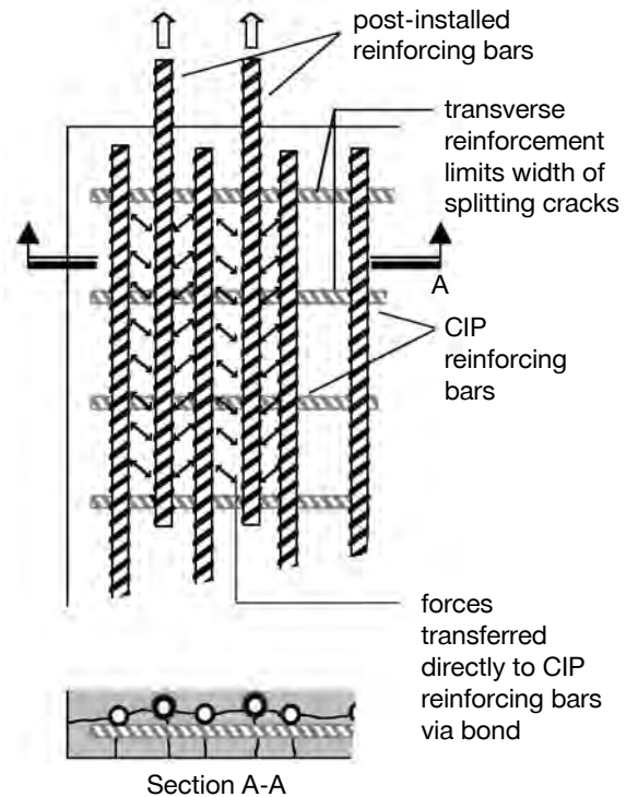
Post-installed reinforcement designed as a lap splice
