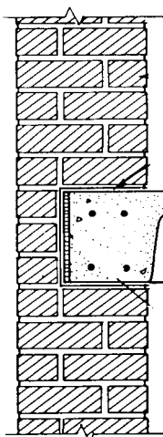
12" Brick Bearing Walls
