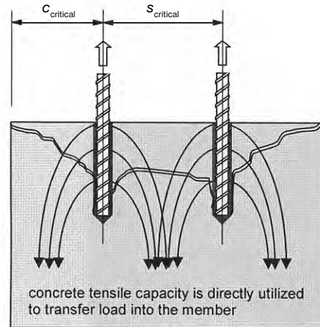
Reinforcing dowels designed using anchor theory
