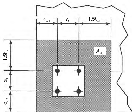
Example of determination of A_{Nc}
