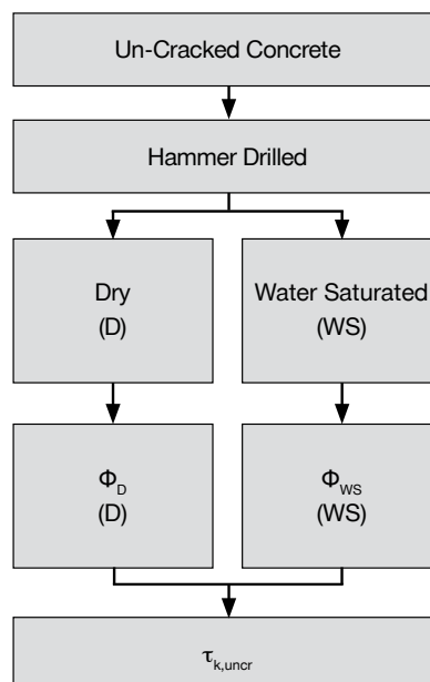
Figure 2 — Flowchart for Establishment of Design Bond Strength
