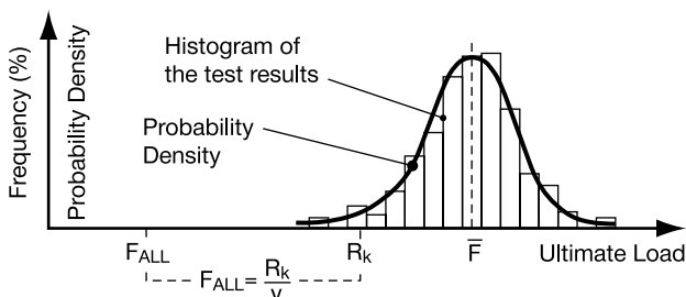
Fig. 2.2.1 Frequency distribution of fastener loads, demonstrating the significance of the 5% fractile and the allowable load
