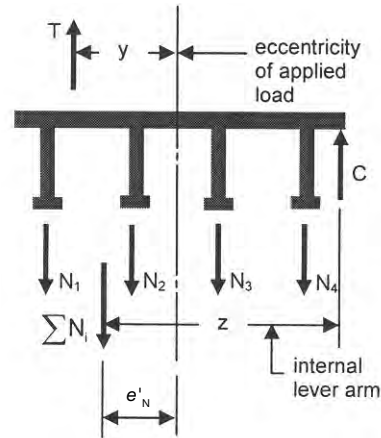
Definition of e'_N for anchor groups
